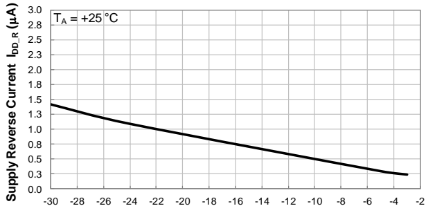
Supply Voltage (V) Reverse Supply Current vs Supply Voltage
