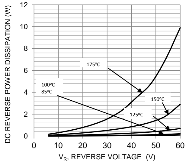
Figure 4 DC Reverse Power Dissipation
