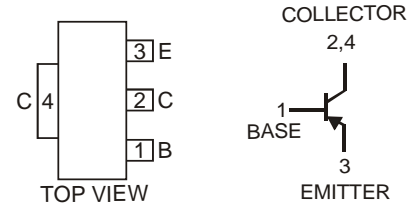
TOP VIEW Schematic and Pin Configuration
