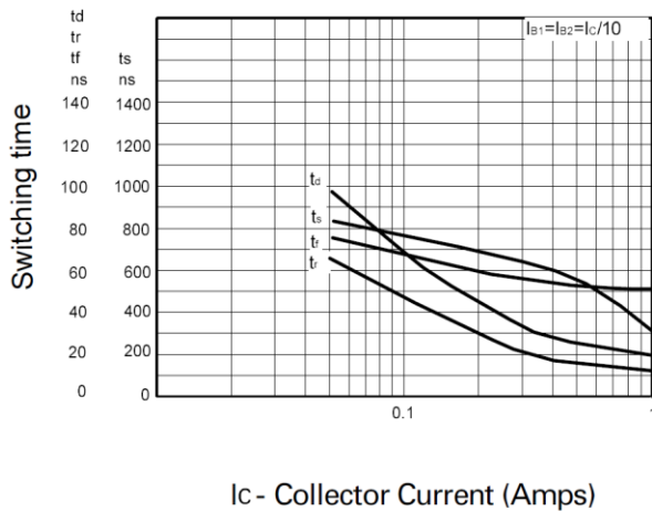
Switching Speeds
