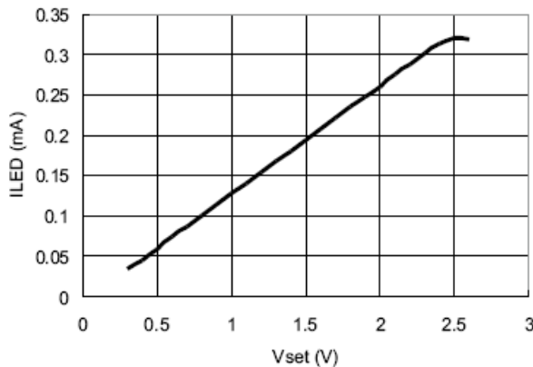
11. I_{LED} VS V_{SET} ( V_{IN} = 16\text{V} , 3 LEDs, 47\mu\text{H} , R_s = 0.15\Omega )
