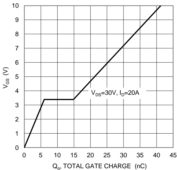
Figure 11. Gate Charge
