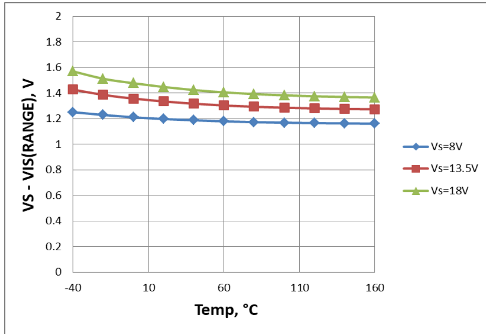
Figure 32. Sense Signal Maximum Voltage V_S - V_{IS(RANGE)} = f(T_J; V_S)
