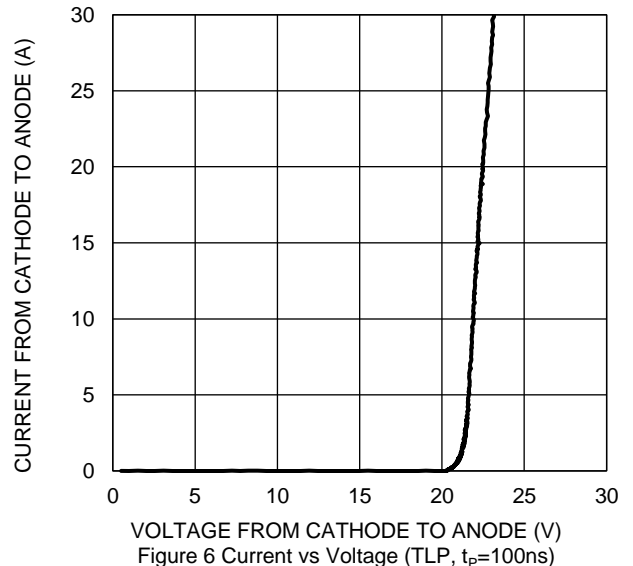
Figure 6 Current vs Voltage (TLP, t p =100ns)
