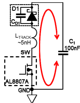
Figure 41 PCB Loop Resonance
