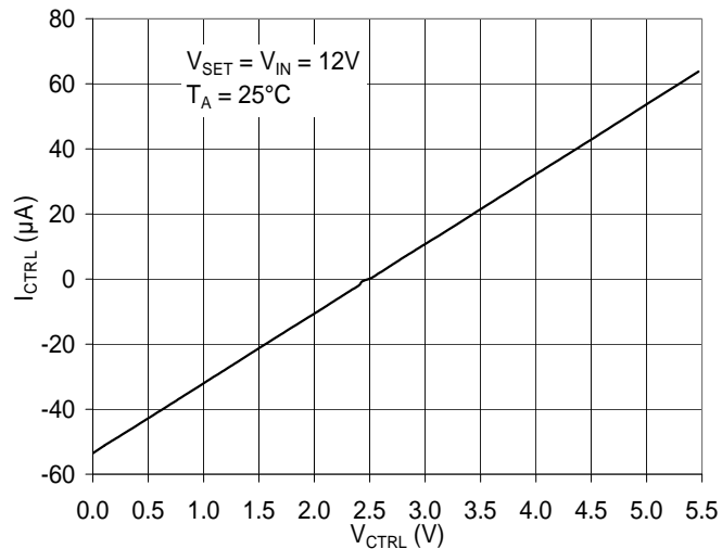
Figure 2 I CTRL vs. V CTRL
