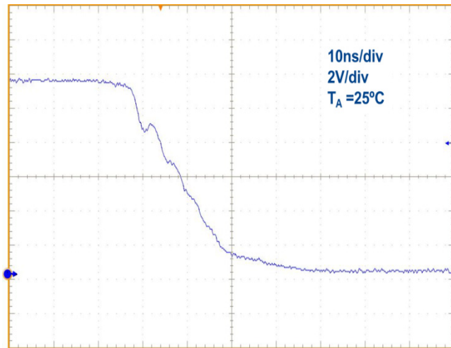
Figure 8 SW Output Fall Time
