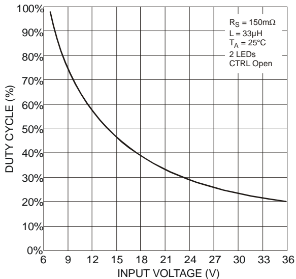
Figure 13 Duty Cycle vs. Input Voltage
