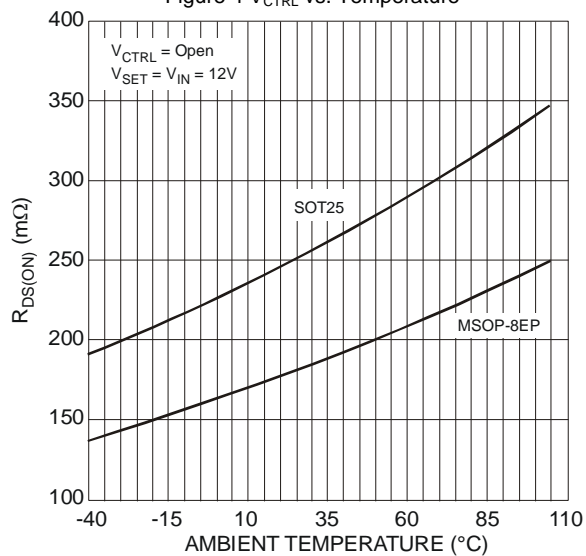
Figure 6 SW R DS(ON) vs. Temperature
