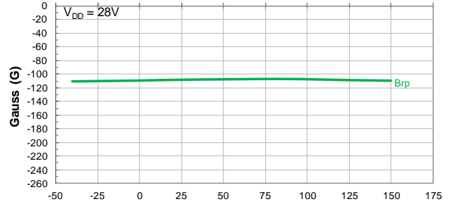
Switch Release Point Brp vs Temperature
