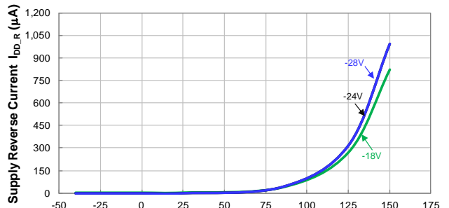
Supply Reverse Current vs Temperature
