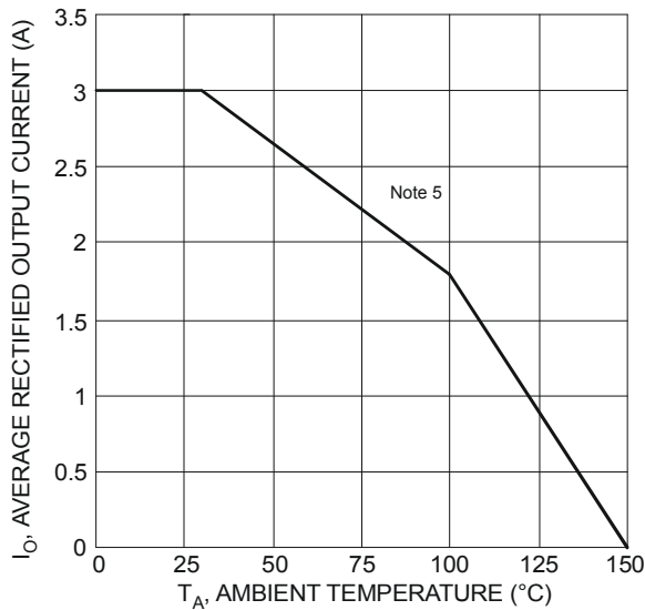
Figure 5 DC Forward Current Derating Curve
