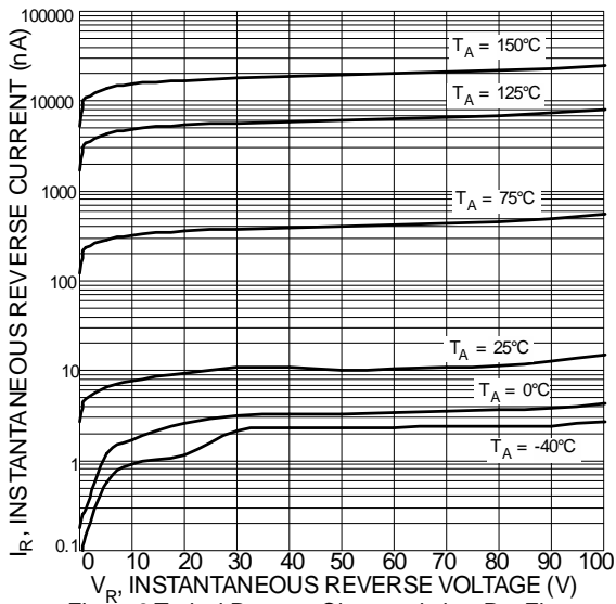
Figure 3 Typical Reverse Characteristics, Per Element
