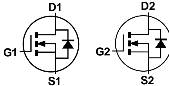
Internal Schematic
