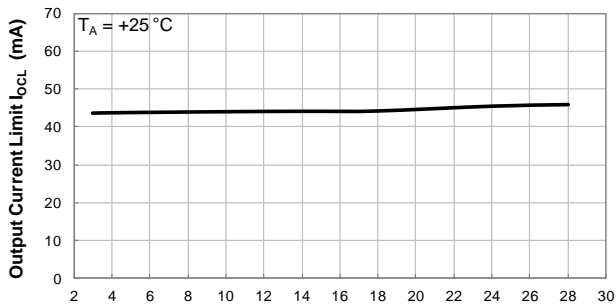
Output Current Limit vs Supply Voltage
