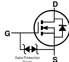
Equivalent Circuit
