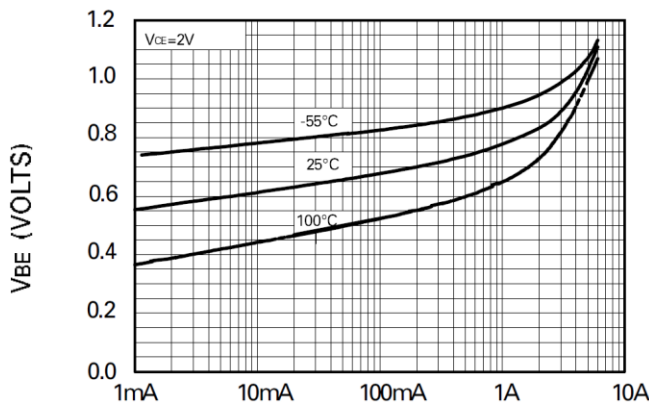
Collector Current
