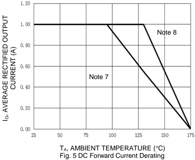
Fig. 5 DC Forward Current Derating
