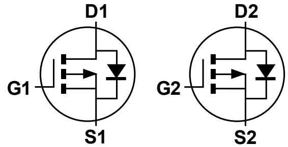
Equivalent Circuit
