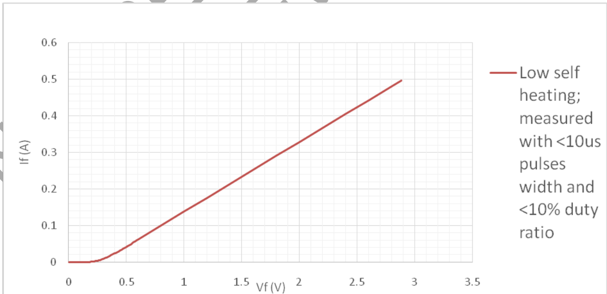
Figure 28. DGD0506 'Internal Diode + Internal Resistor' V_f vs. I_f
