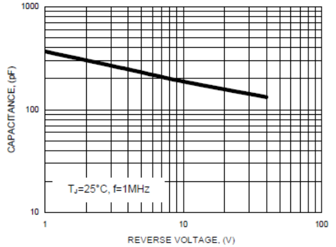
FIG.4-TYPICAL TOTAL CAPACITANCE
