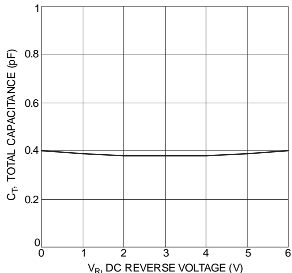
Figure 6 Typical Total Capacitance, I/Os
