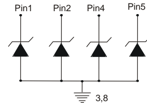
Device Schematic
