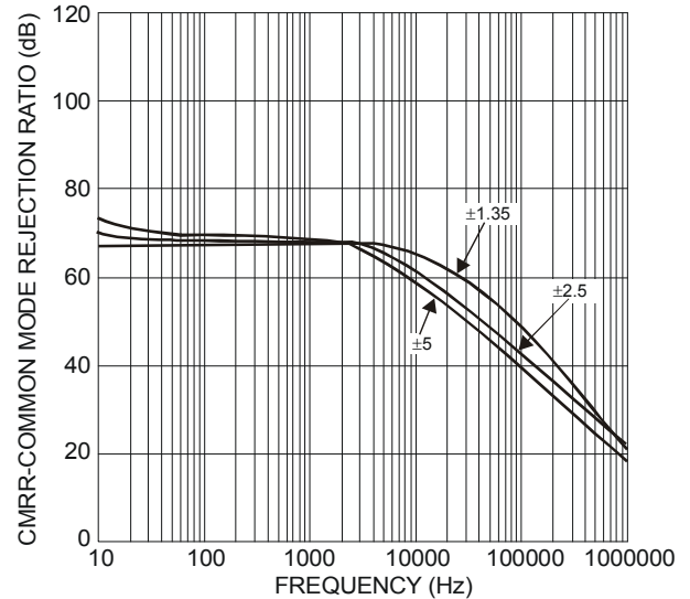
Figure 6 Common Mode Rejection Ratio vs. Frequency
