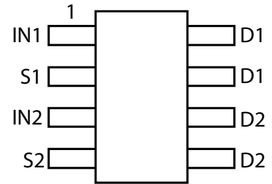
Top view Pin-Out
