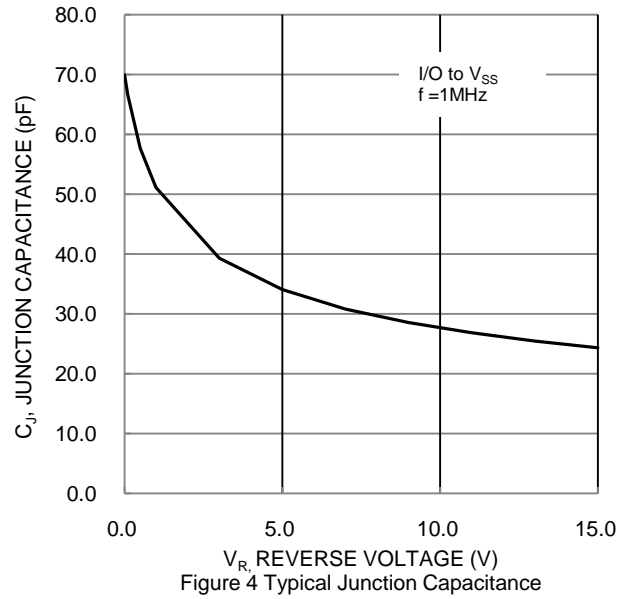
Figure 4 Typical Junction Capacitance
