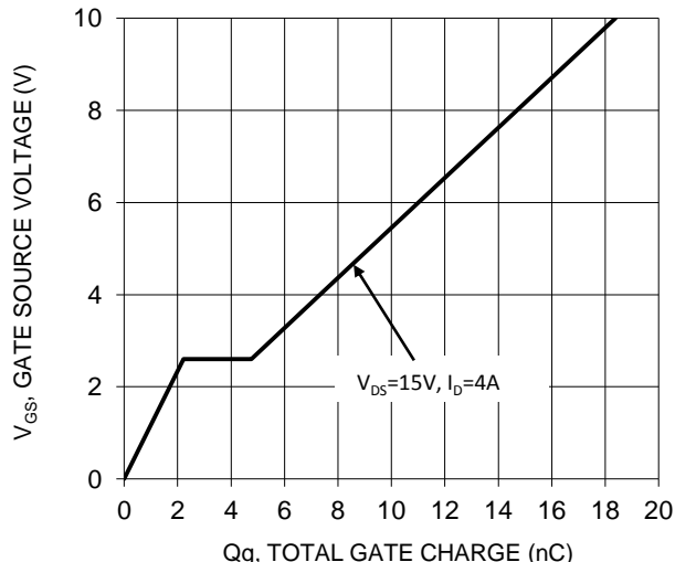
Figure 12 Gate Charge
