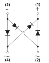
Internal Schematic
