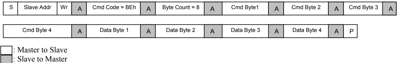
Figure 7-2 SMBus Block Write Command Format, to Write to a PI7C9X2G608GP Register without PEC
