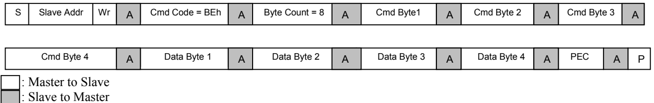
Figure 7-3 SMBus Block Write Command Format, to Write to a PI7C9X2G608GP Register with PEC
