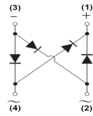
Internal Schematic
