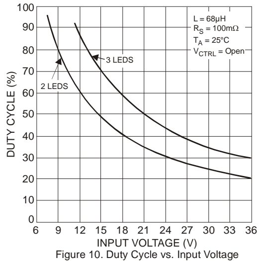
Figure 10. Duty Cycle vs. Input Voltage
