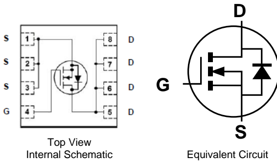
Equivalent Circuit
