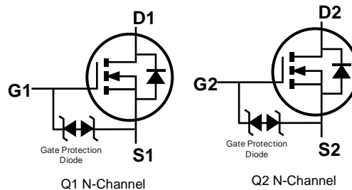
Equivalent Circuit
