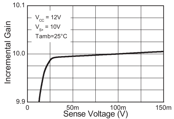
Incremental Gain v Sense Voltage
