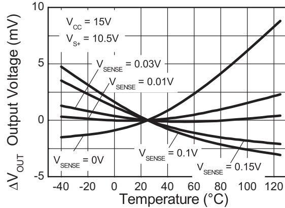
Temperature Characteristic
