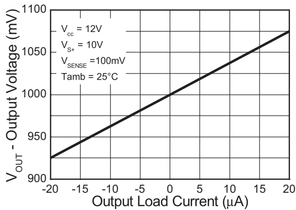
V_{OUT} v Load Current
