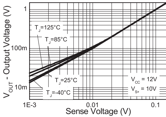
Output Voltage v Sense Voltage
