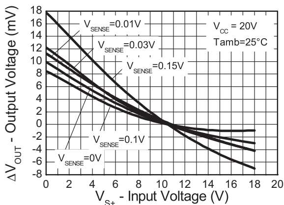
Common Mode Characteristic
