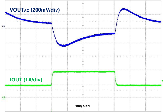
Figure 41. Load Transient, I_{OUT} = 1\text{A} to 2\text{A} to 1\text{A}
