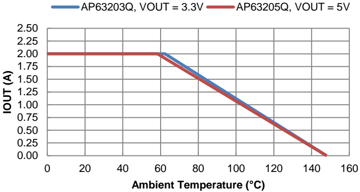
Figure 76. Output Current Derating Curve vs. Ambient Temperature, AP63203Q/AP63205Q, VIN = 12V
