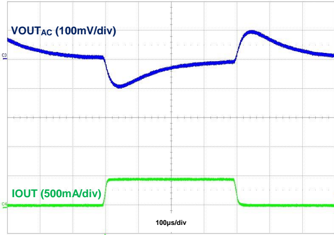
Figure 40. Load Transient, I_{OUT} = 50\text{mA} to 500\text{mA} to 50\text{mA}
