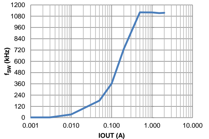
Figure 48. fsw vs. Load
