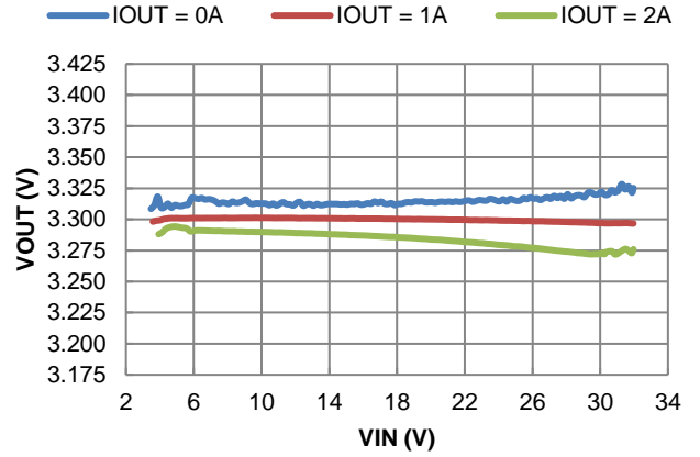
Figure 44. Line Regulation
