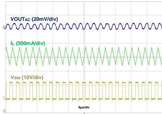
Figure 23. Output Voltage Ripple, V_{OUT} = 5\text{V} , I_{OUT} = 2\text{A}
