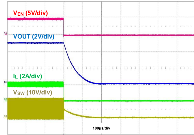
Figure 70. Shutdown using EN, IOU = 2A
