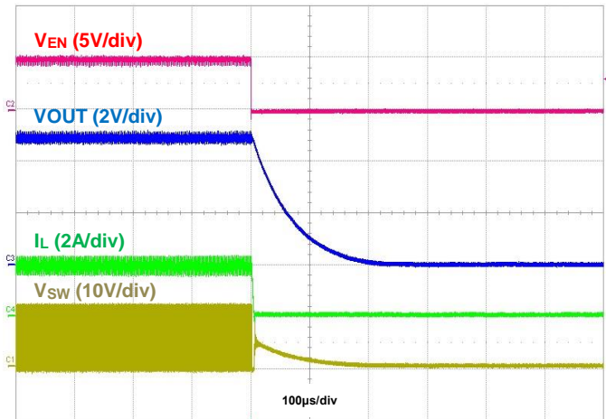
Figure 12. Shutdown using EN, I_{OUT} = 2\text{A}
