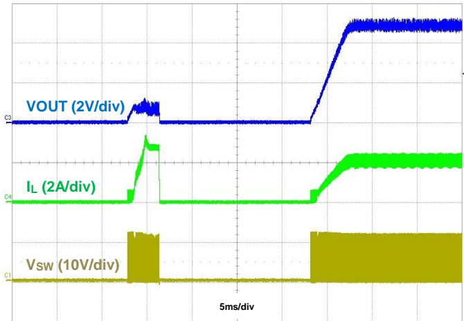
Figure 14. Output Short Recovery, I_{OUT} = 2\text{A}
