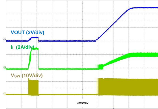
Figure 72. Output Short Recovery, IOU = 2A
