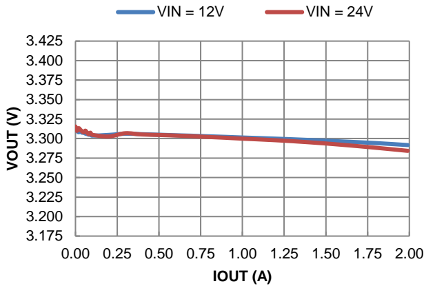
Figure 45. Load Regulation
