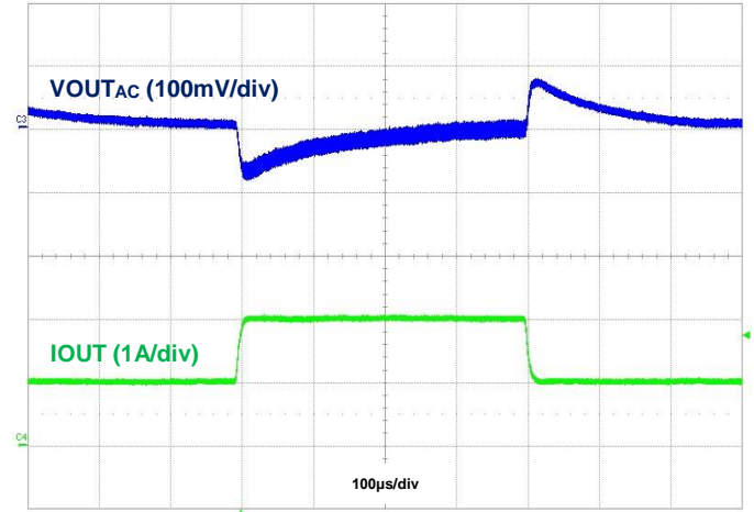
Figure 52. Load Transient, I_{OUT} = 1\text{A} to 2\text{A} to 1\text{A}
