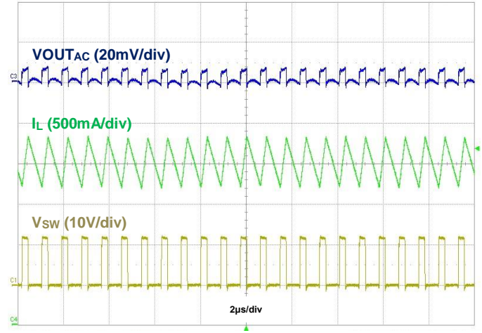
Figure 50. Output Voltage Ripple, I_{OUT} = 2\text{A}
