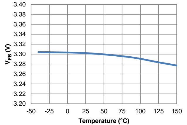
Figure 46. Feedback Voltage vs. Temperature, IOUT = 1A
