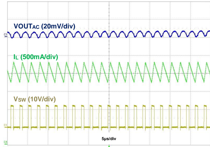
Figure 25. Output Voltage Ripple, V_{OUT} = 3.3\text{V} , I_{OUT} = 2\text{A}
