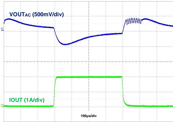
Figure 42. Load Transient, I_{OUT} = 50\text{mA} to 2\text{A} to 50\text{mA}
