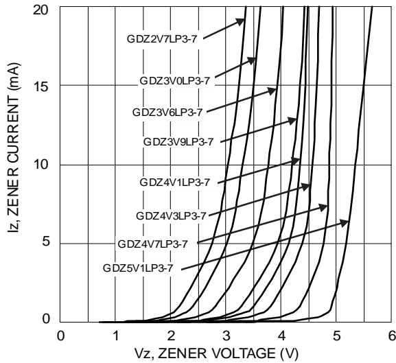
Figure 3 Typical Zener Breakdown Characteristics, GDZ2V7LP3 – GDZ5V1LP3
