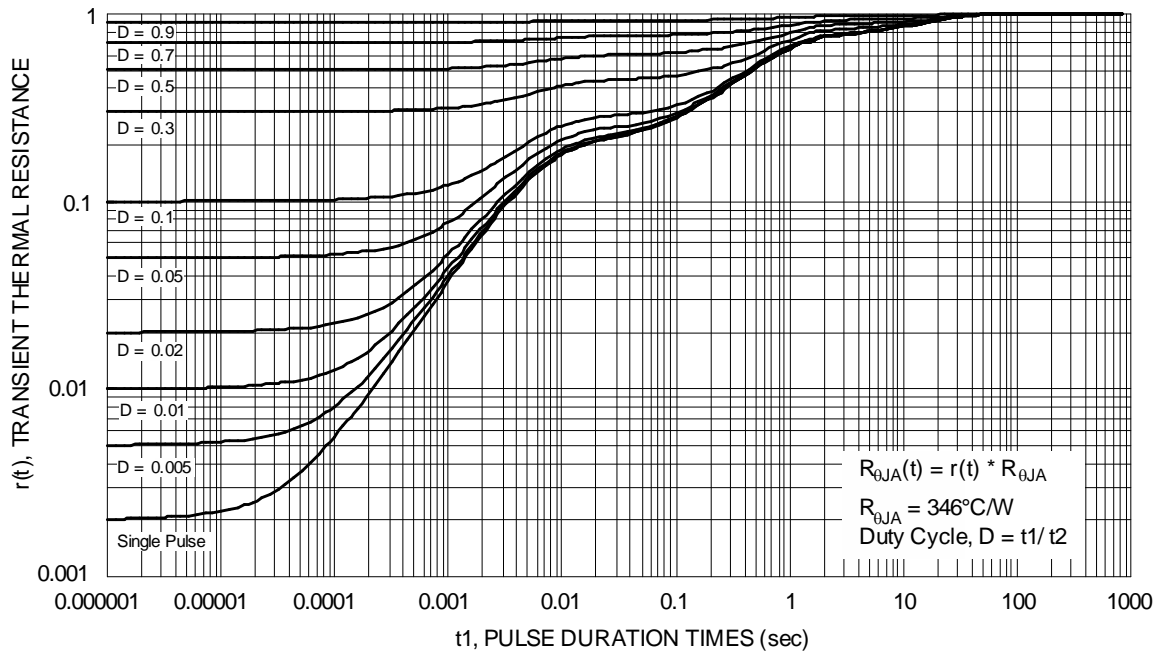
Figure 15 Transient Thermal Resistance
