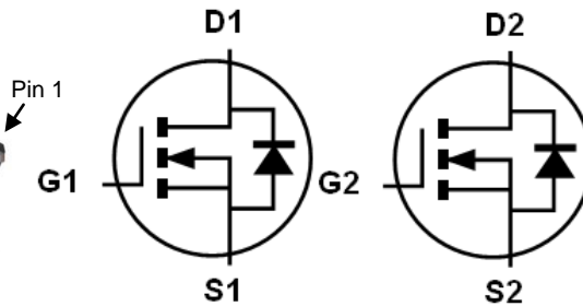
Equivalent Circuit
