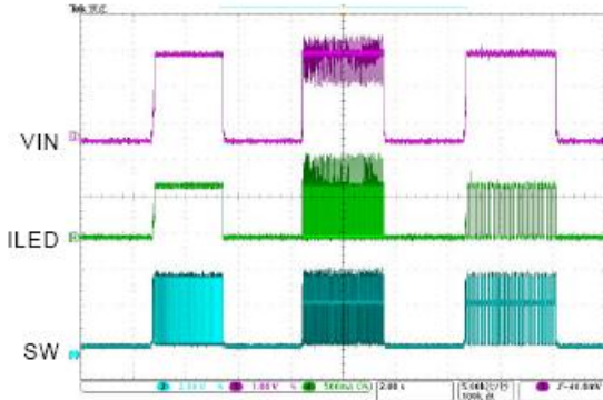
5. 3 Modes Change
