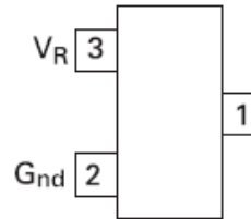
SOT23 Package Suffix - F
