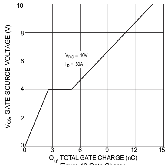
Figure 12 Gate Charge
