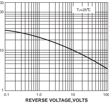
FIG. 5-TYPICAL JUNCTION CAPACITANCE
