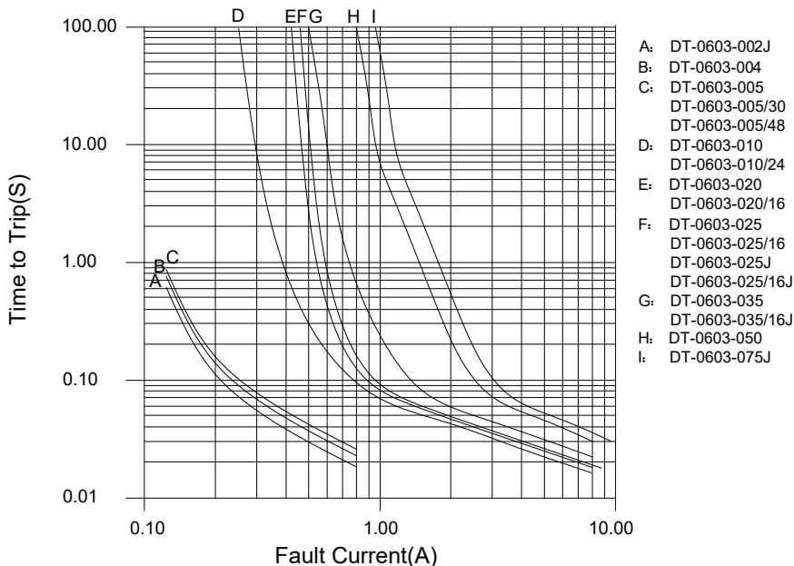
0603 Series TTT Vs Fault current chart
