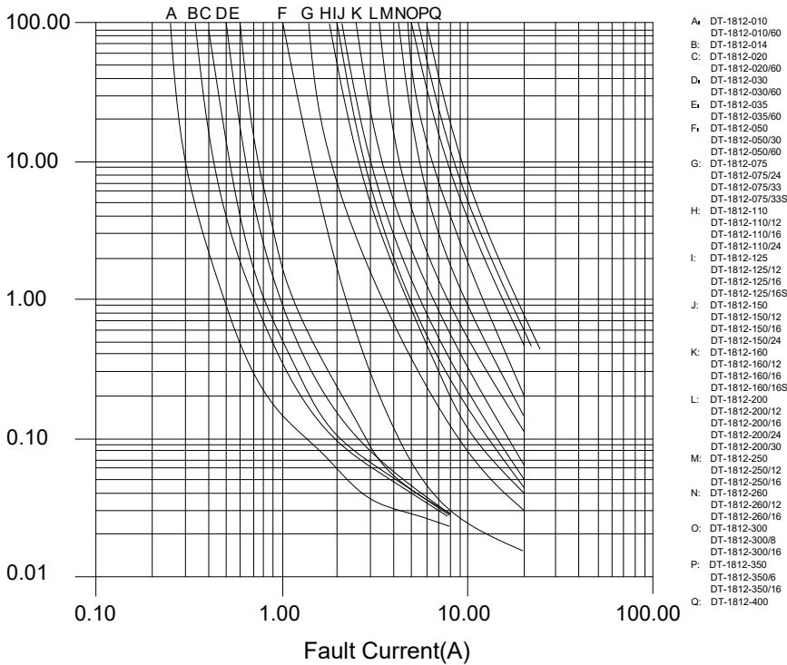
1812 Series TTT Vs Fault current chart
