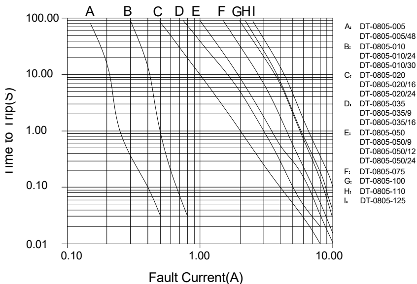
0805 Series TTT Vs Fault current chart
