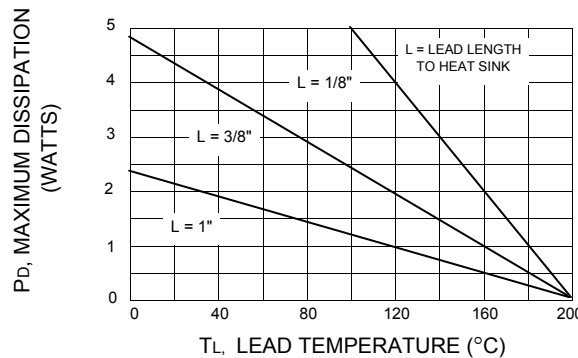
Fig. 1 Power Temperature Derating Curve
