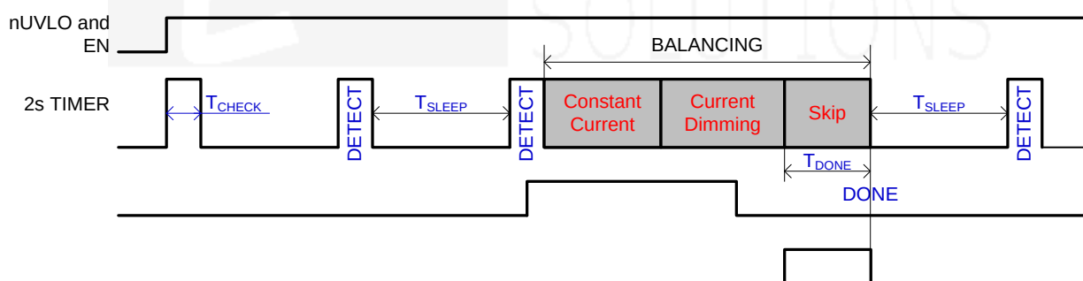
Figure 4: Timing Profile
