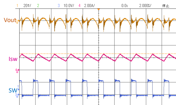
Switching Waveform at Iout = 2A ( V_{in}=12\text{V} , V_{out}=3.3\text{V} )
