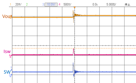
Switching Waveform at Iout = 0A ( V_{in}=12\text{V} , V_{out}=3.3\text{V} )
