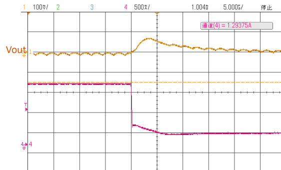
Load Transient Response – I out Falling Edge 1A/0.2 \mu s Vin=12V, Vout=1.1V, L=2.2 \mu H, Cout=22 \mu Fx2, Iout 1.5-0.3A
