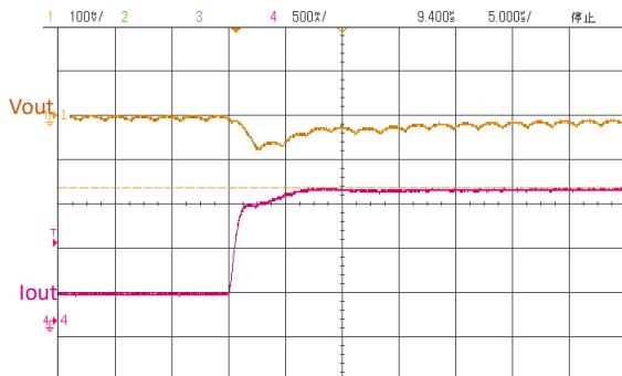
Load Transient Response – I out Rising Edge 1A/1 \mu s Vin=12V, Vout=1.1V, L=2.2 \mu H, Cout=22 \mu Fx2, Iout 0.3-1.5A
