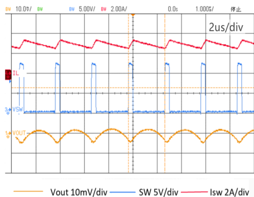
Waveform 1.2V/3A V_{IN}=12\text{V}
