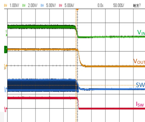
Shut Down from VIN V_{IN}=3.3\text{V} , V_{OUT}=1.2\text{V} , I_{OUT}=4\text{A}
