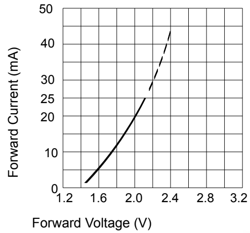
Forward Current vs. Forward Voltage (Ta=25 )
